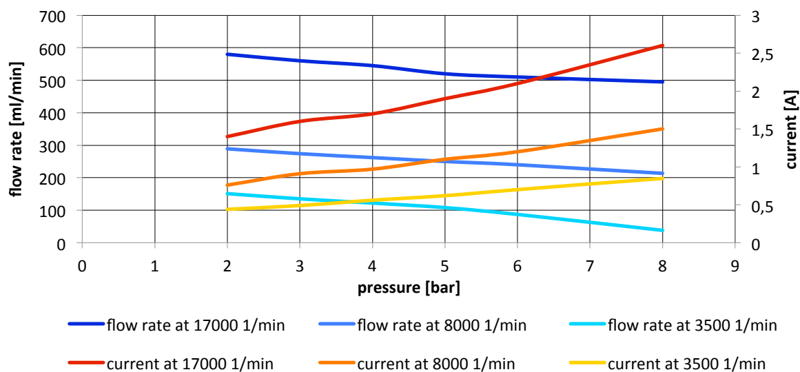
Characteristic at 7,0V
