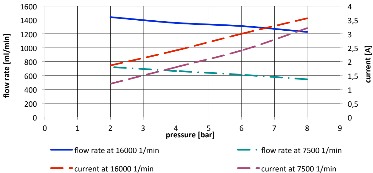
Characteristic at 12,0V
